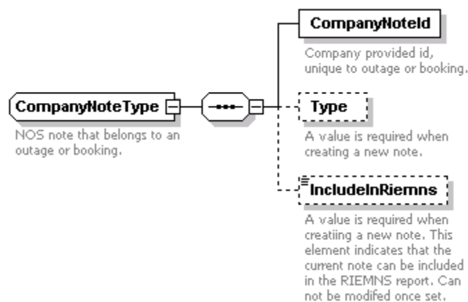
Figure 2-1 IncludedInRiemns element
